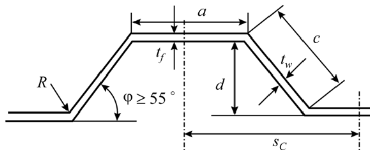
Fig 28: Dimensions of a corrugated bulkhead
