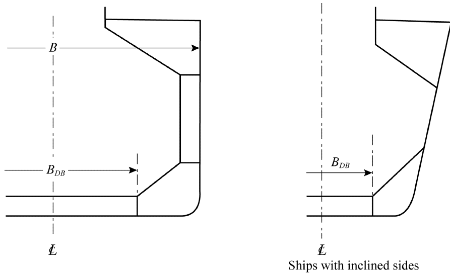
Fig 17: Breadth of double bottom
