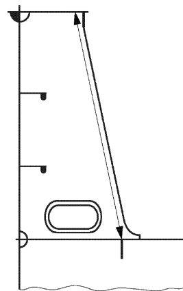
Fig 5: Coaming stay: example 4
