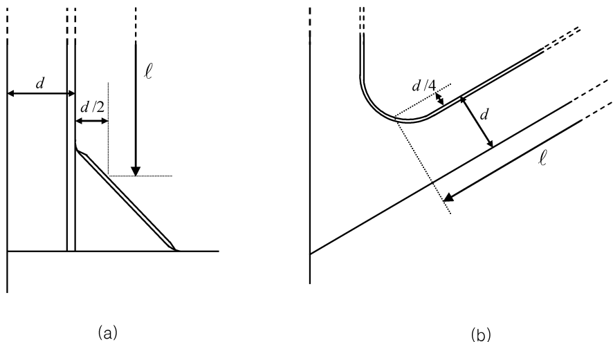
Fig 13 : Span of primary support member
