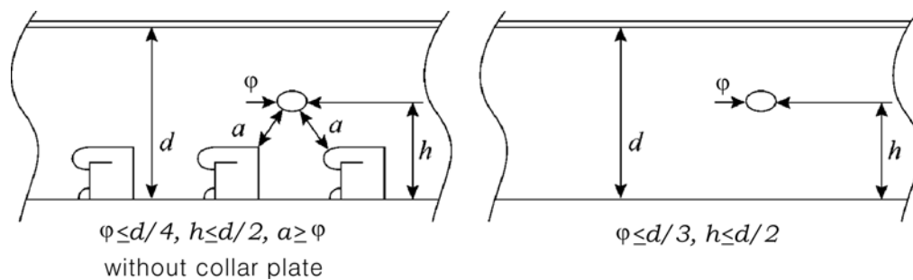
Fig 15: Location and dimensions of lightening holes
