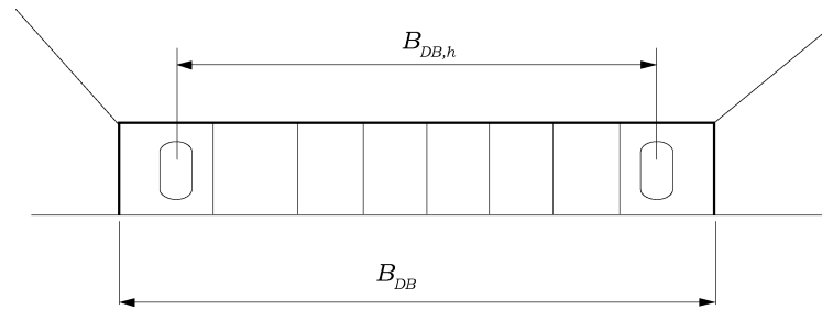
Fig 3: Dimensions B_{DB} and B_{DB,h}
