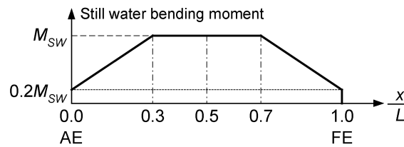
Fig 2: Preliminary still water bending moment distribution
