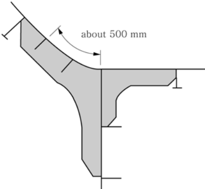
Fig 8: Example of insertion of transverse rib
