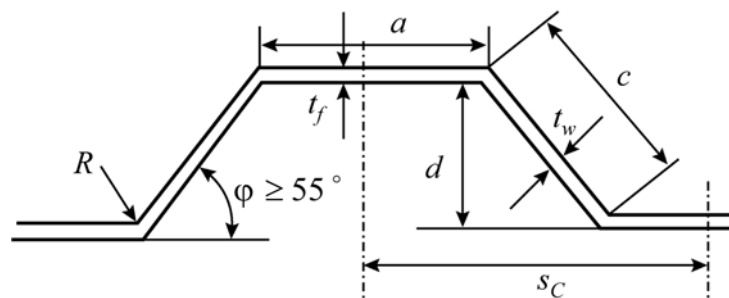
Fig 1: Corrugated bulkhead
