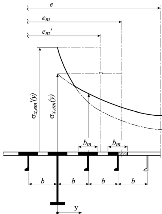
Fig 3: Stiffening parallel to web
