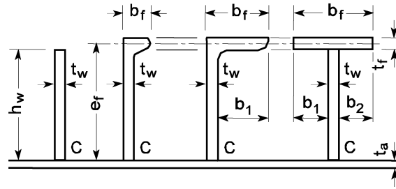
Fig 2: Dimensions of stiffeners
