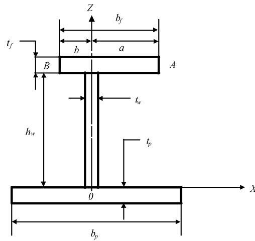
Fig 1: Sectional parameters of a stiffener
