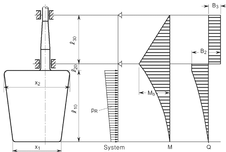
Fig 6: Spade rudder
