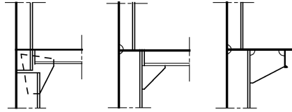
Fig 1: End attachment of superstructure frames
