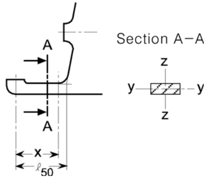
Fig 13: Sole piece
