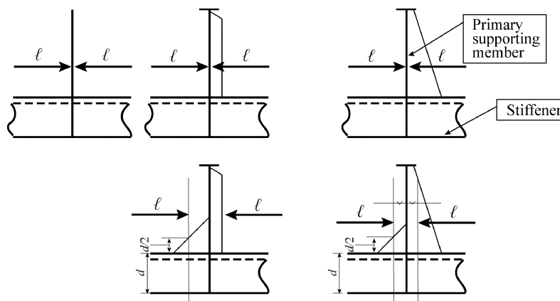
Fig 2: Span of ordinary stiffeners
