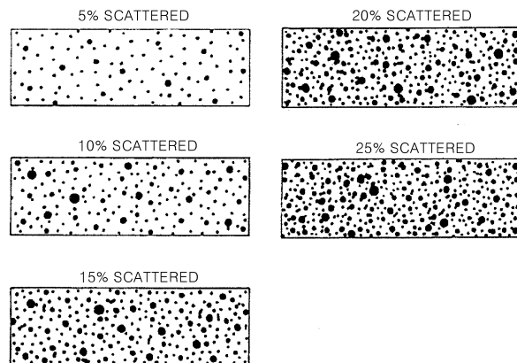
Fig 1: Pitting intensity diagrams (from 5 % to 25 % intensity)
