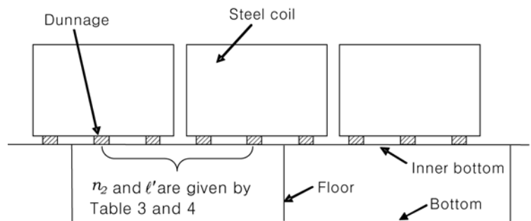
Fig 3: Loading condition of steel coils (example of n_2=4 , n_3=3 )
