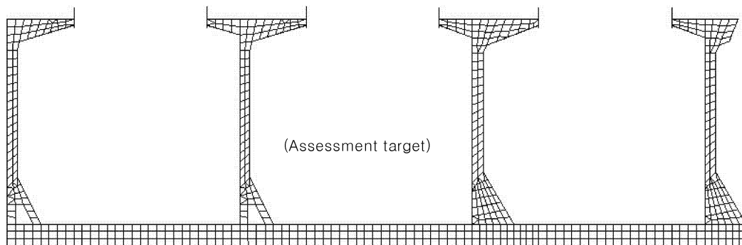
Fig 1: Longitudinal extent of the finite element model
