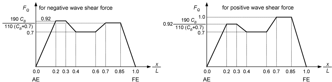
Fig 4: Distribution factor F_Q
