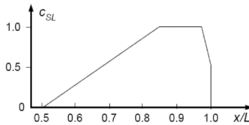
Fig 7: Distribution Factor c_{SL}
