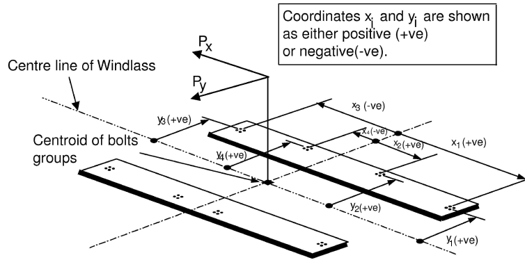
Fig 3: Sign convention
